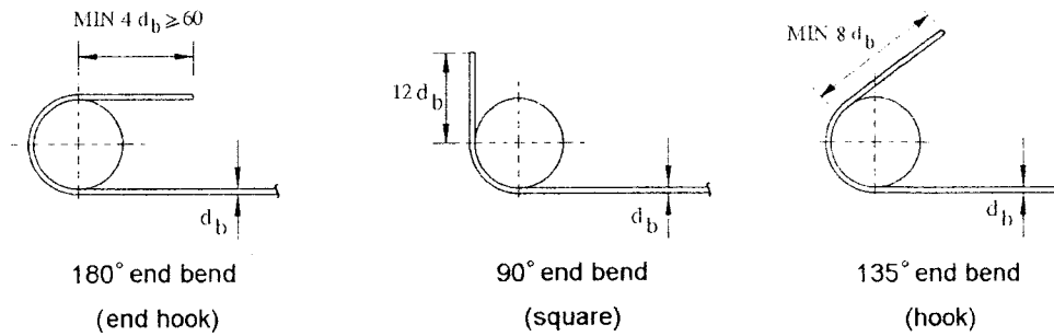
Standard hooks for reinforcement (Excluding stirrups)
